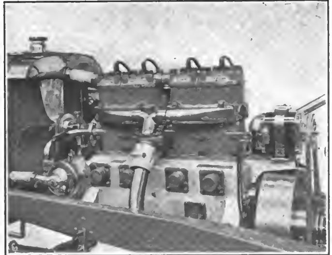
Carburetor side of Delaunay-Belleville motor
